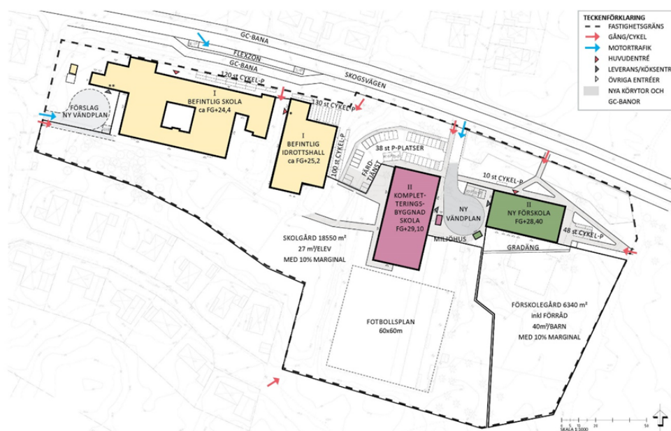
Figur 18 Situationsplan (Ramboll).
