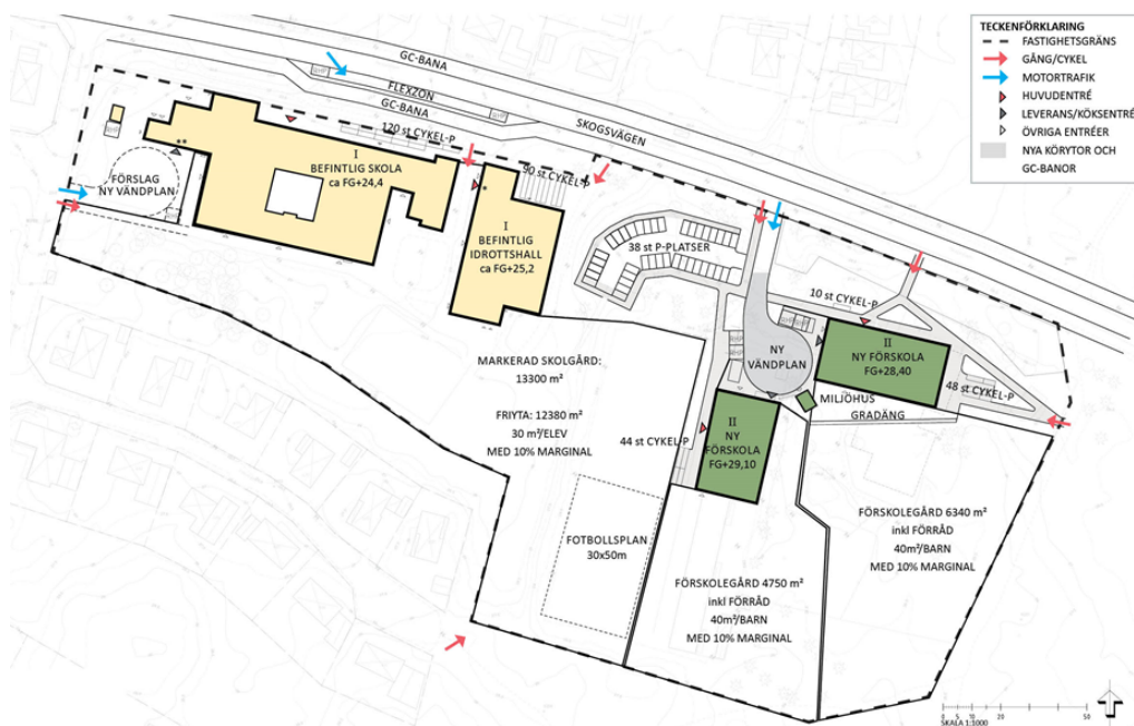
Figur 15 Situationsplan (Ramboll).
